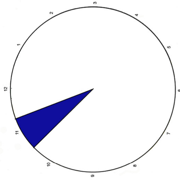
Paleozoic
