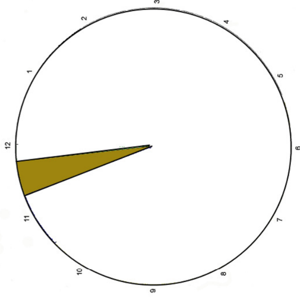
Mesozoic
