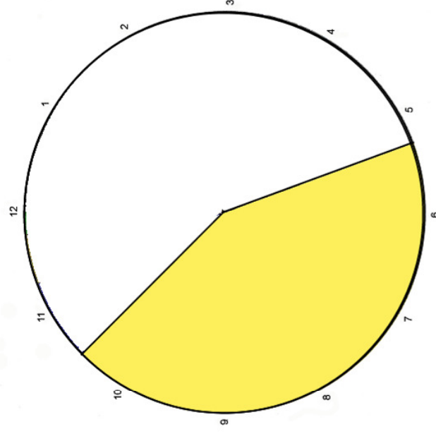
Proterozoic
