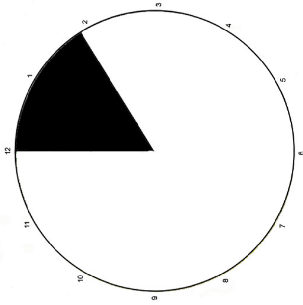
Hadean
